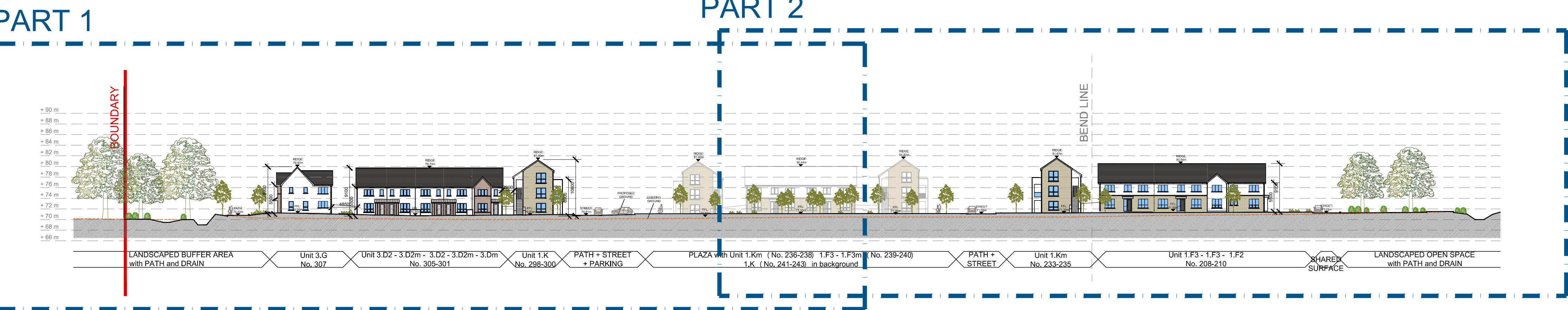
PROPOSED SITE SECTION FF - scale 1:500
