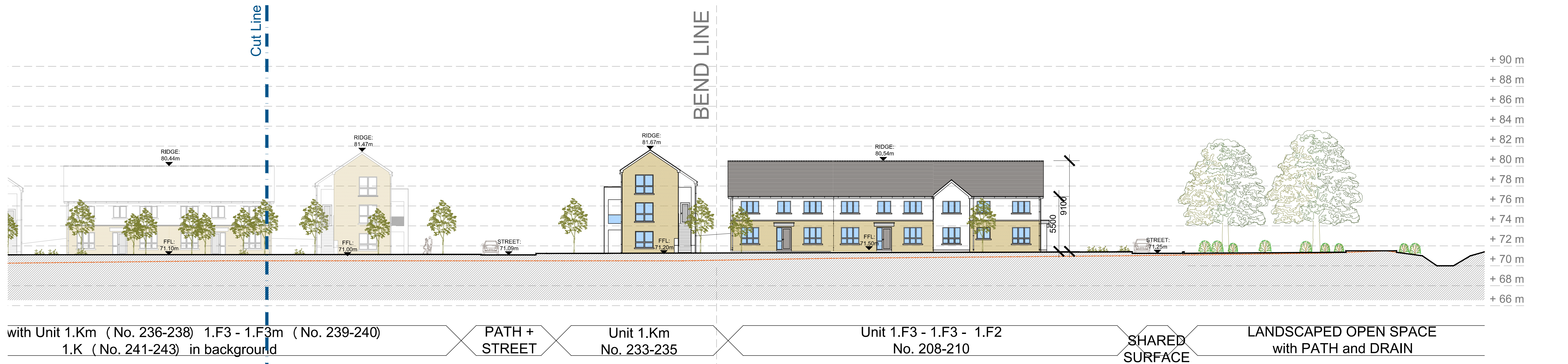
PROPOSED SITE SECTION FF (Part 1) - scale 1:200
